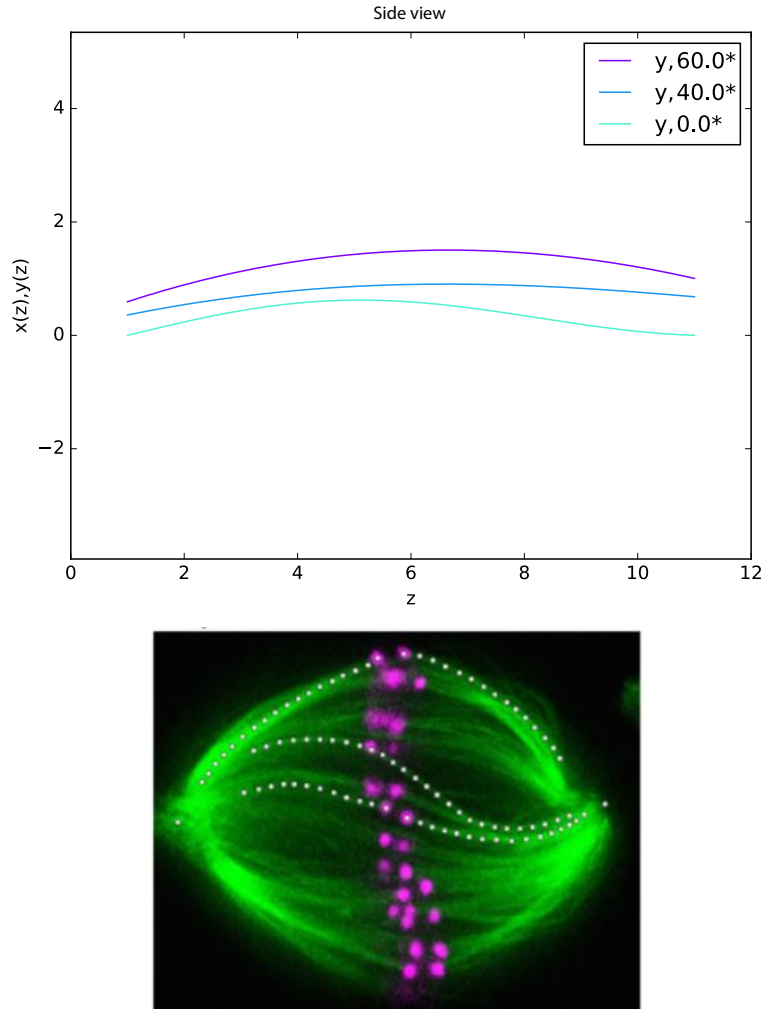
Figure 89: Example of first-order model predictions, side view, along with experimental spindle images ([43]). Obtained for the choice of parameters m_0^\perp = -25.0 \text{ pN}\mu\text{m} , m_0^\parallel = -10.0 \text{ pN}\mu\text{m} , m_1^\perp = 1.0 \text{ pN}\mu\text{m} , m_1^\parallel = 350.0 \text{ pN}\mu\text{m} , \alpha_0 = \pi/3 , \theta_a = 0.01 , \theta_b = \pi/3 . Figure axis units are \mu\text{m} .
