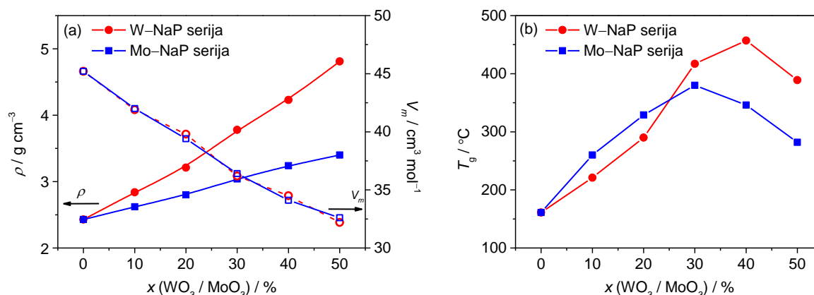
Slika 59. Ovisnost (a) gustoće, \rho , i molarnog volumena, V_m , i (b) temperature staklišta, T_g , o množinskom udjelu \text{WO}_3 i \text{MoO}_3 u serijama stakala x\text{WO}_3-40\text{Na}_2\text{O}-(60-x)\text{P}_2\text{O}_5 i x\text{MoO}_3-40\text{Na}_2\text{O}-(60-x)\text{P}_2\text{O}_5 , x = 0-50\% .
