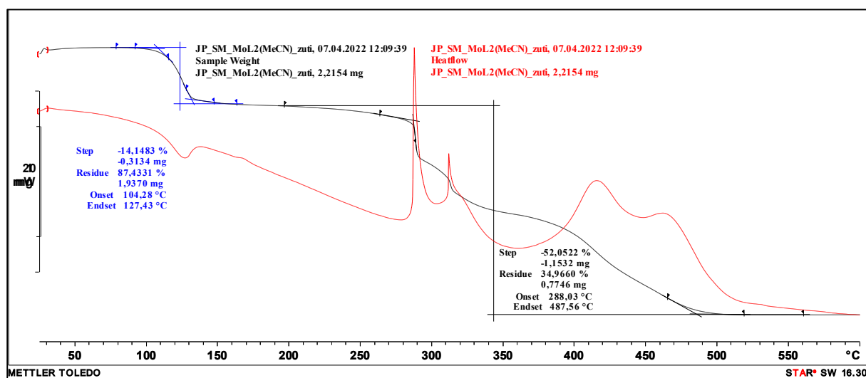
Slika D21. Termogram kompleksnog spoja [\text{MoO}_2(\text{L}^2)(\text{H}_2\text{O})] \cdot \text{MeCN}
