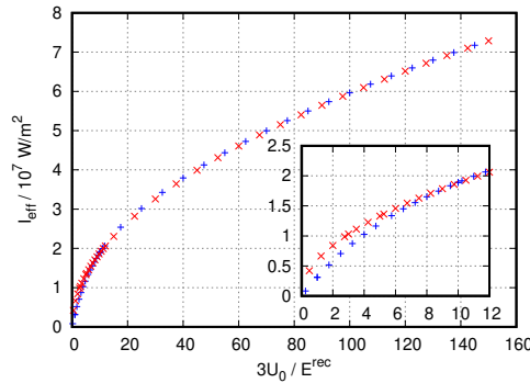
Fig. 8. The total effective intensity I_{\text{eff}} experienced by the atoms trapped in the motional ground state of a 3D blue-detuned magic wavelength optical lattice. I_{\text{eff}} values were calculated for Wannier-Stark (Wannier) states for the vertical (horizontal) directions in the optical lattice (blue crosses) and Gaussian states (red crosses) in a harmonic potential approximation.
