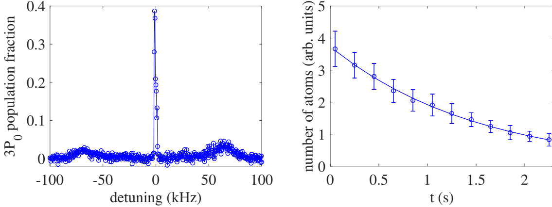
Figure 2.7: (left) Sideband spectroscopy of the clock transition for lattice depth of 85 E_r giving an axial lattice temperature of about 15 \mu\text{K} . The central peak corresponds to the clock transition frequency. Blue points represent the population fraction in the excited clock state as a function of clock laser detuning from the clock resonance. The blue line was added for better visual clarity of the central resonance. (right) Lifetime of atoms in the trap. Blue points on the right figure represent the number of atoms in the trap as a function of time atoms spent in the trap. An exponentially decaying function, represented by solid blue line, was fitted to the data set. We find the lifetime of atoms in the lattice to be equal to 1.5(1) seconds.
