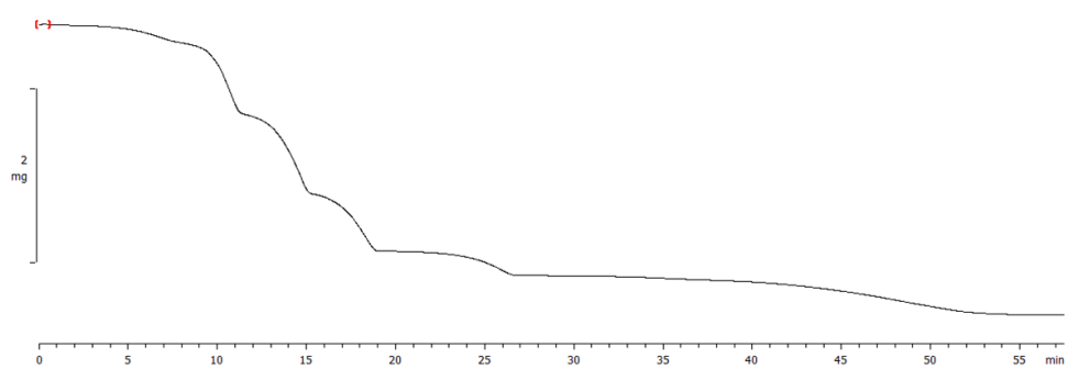
Slika D55. TG krivulja kokristala soli \text{CuCl}(\text{phen})_2\text{Cl}(\text{13tfib})_4
