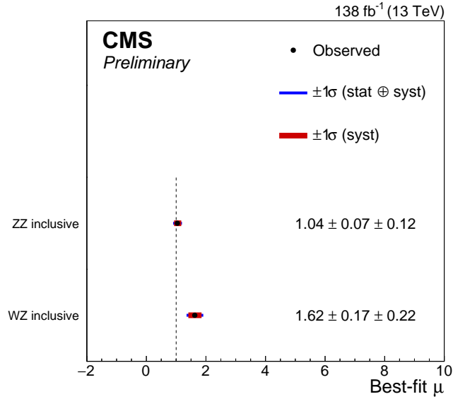
Figure 5.1: Result of the VZ, Z \rightarrow b\bar{b} channel analysis using the full Run 2 dataset for both the WZ and ZZ production modes
