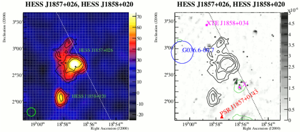
Figure 5.1: Left: VHE gamma-ray image of HESS J1858+020 and a larger nearby source J1857+026. Right: The HESS significance contours (black) and X-ray contours (green) overlaid on a radio image (grey-scale). Figures are taken from Aharonian et al. (2008) .
