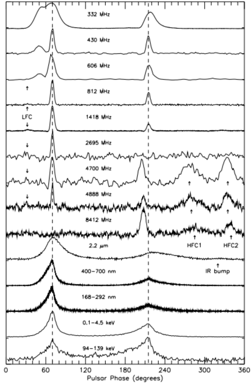
Figure 1.12: Crab pulsar profiles throughout the spectrum (from radio to X-rays). Figure is taken from Moffett & Hankins (1996) .
