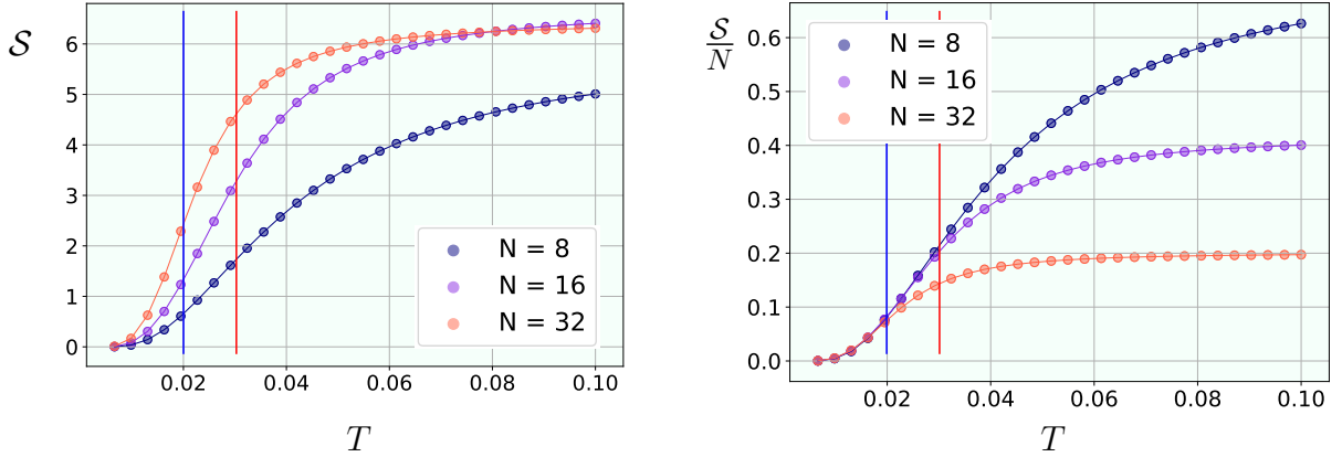
Figure 6.25: Von Neumann entropy \mathcal{S} (left) and scaled Von Neumann entropy \mathcal{S}/N (right) as a function of temperature T , computed for Rydberg atom model model at the point of maximal entanglement \tilde{\Omega} = 0.05 for different system sizes. As a consequence of truncation error, for N = 16 we expect the accurate results up to T \approx 0.03 (red line), and for N = 32 up to T \approx 0.02 (blue line). We observe the agreement of the scaled Von Neumann curves up to the temperature of the predicted accuracy decrease. For N = 8 there is no truncation error. Temperature T is expressed in units of J/k_B .
