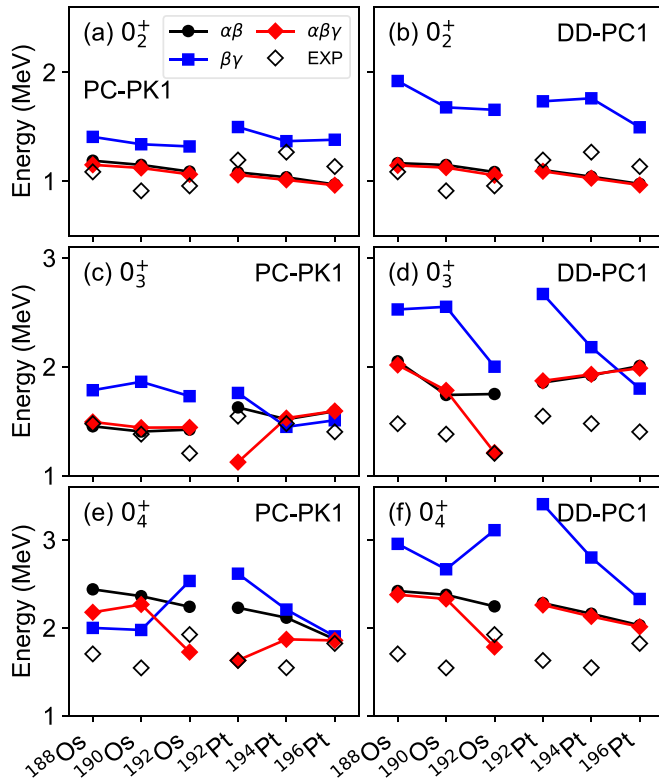
FIG. 8. Excitation energies of the three lowest 0^+ excited states in ^{188,190,192}\text{Os} and ^{192,194,196}\text{Pt} , obtained from IBM calculations that include the 2D [triaxial quadrupole ( \beta, \gamma )], 2D (axial quadrupole \beta plus pairing \alpha ), and 3D [triaxial quadrupole ( \beta, \gamma ) and pairing \alpha ] degrees of freedom, in comparison with the corresponding experimental levels.
