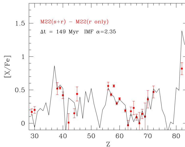
Figure 1. Average abundances observed in the globular cluster M22 (red points) compared to the theoretical expectations deduced from stellar models (from [9]).
