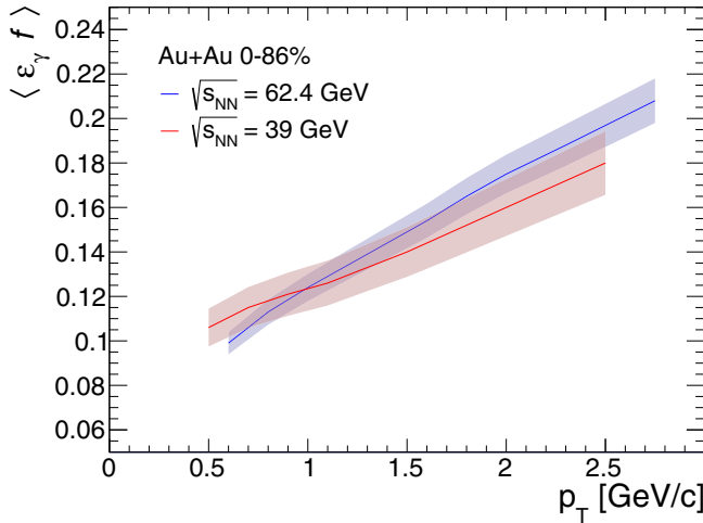
FIG. 6. Simulated conditional probability, \langle \epsilon_\gamma f \rangle , to detect the second photon from a \pi^0 decay in the MB data samples at \sqrt{s_{NN}} = 39 and 62.4 GeV. The x axis is the p_T of the e^+e^- pair.
