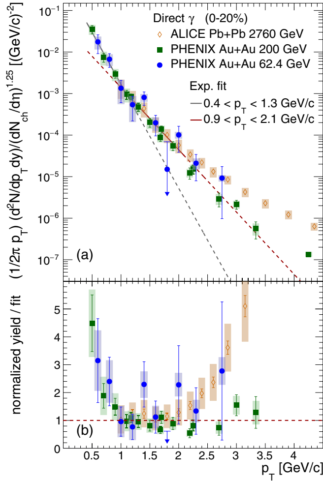
FIG. 11. Direct-photon yield normalized to (dN_{ch}/d\eta)^{1.25} in the low- p_T region for 0%–20% centrality in Pb+Pb at 2760 GeV, Au+Au at 200 GeV, and Au+Au at 62.4 GeV. (a) gives the normalized yield and two exponential fits to the data in the p_T region below 1.3 GeV/c and from 0.9 to 2.1 GeV/c. The dashed line extrapolates the fits beyond the fit ranges. (b) shows the ratio of the data sets to the fit in the range 0.9 to 2.1 GeV/c range.
