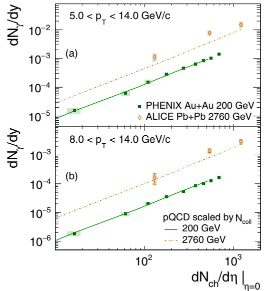
FIG. 15. Integrated direct-photon yields from A + A collisions for p_{T,\text{min}} of 5 GeV/ c (a) and 8 GeV/ c . The representation is the same as in Fig. 13. Also shown are the results from pQCD calculations scaled by N_{\text{coll}} .
