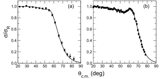
Fig. 3. (a) 136 MeV ^{17}\text{Ne} + ^{208}\text{Pb} elastic scattering angular distribution. (b) 131 MeV ^{20}\text{Ne} + ^{208}\text{Pb} [49] elastic scattering angular distribution. The solid curves denote the optical model fits described in the text.
