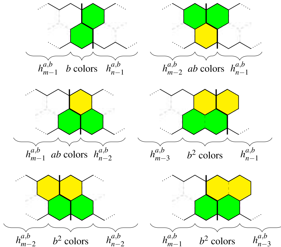
Figure 1.12: Layouts that can occur if tiling is not breakable at position m .
