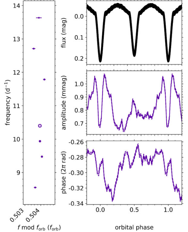
Figure C4. Tidally perturbed pulsation with frequency f = 10.399706(2)d^{-1} .
