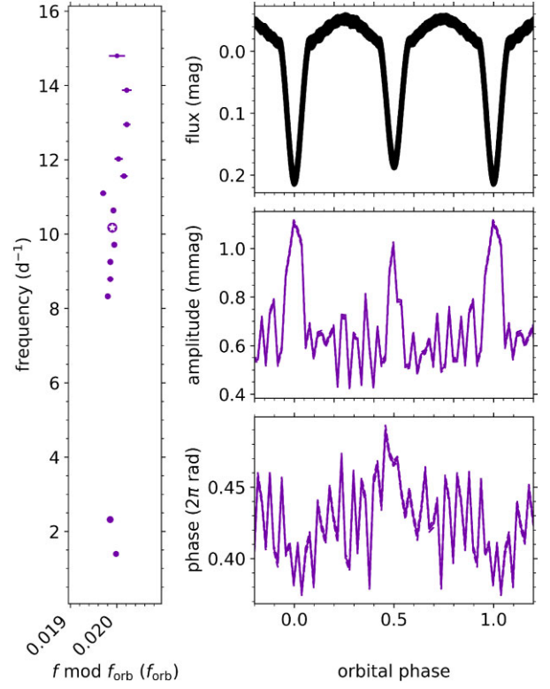
Figure C3. Tidally perturbed pulsation with frequency f = 10.176017(2)d^{-1} .
