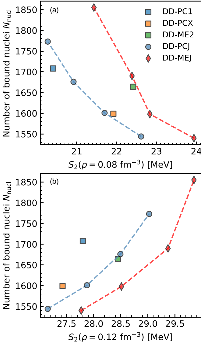
FIG. 5. The total number of bound nuclei N_{\text{nuc1}} shown as a function of the symmetry energy S_2 at \rho = 0.08 \text{ fm}^{-3} (a) and \rho = 0.12 \text{ fm}^{-3} (b). Results for DD-PCJ (blue) and DD-MEJ families of EDFs are shown with dashed lines, together with results for DD-PC1, DD-PCX, and DD-ME2 functionals (squares).
