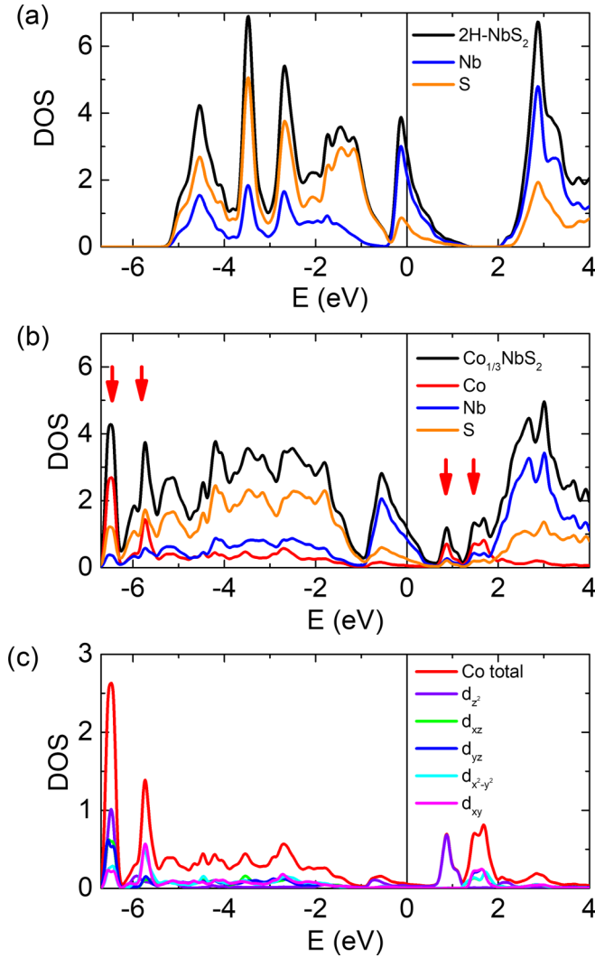
FIG. 9. The density of states (DOS) as calculated for (a) 2H-NbS_2 , (b) Co_{1/3}NbS_2 , and (c) projected on different Co orbitals. Red arrows in (b) mark positions where most of the Co DOS is positioned. To keep the graphs for two compounds easily comparable, the units used in graphs correspond to the number of states per unit energy per unit cell divided by the number of Nb atoms within the unit cell. The origin of the energy scale is set to E_F .
