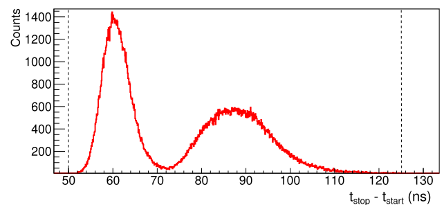
Fig. 3 FF ToF spectrum. The dashed lines indicate the gate applied to identify a fission event
