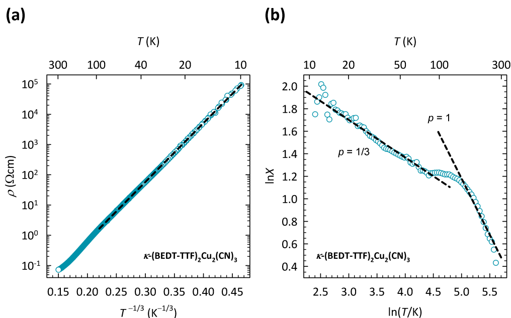
Figure 2. (a) Temperature dependence of resistivity for \kappa -(BEDT-TTF) 2 Cu 2 (CN) 3 on a \log\rho-T^{-1/3} plot. Black dashed line is a fit to the 2D VRH mechanism \rho(T) \propto \exp(T_0/T)^{1/3} . (b) Temperature dependence of the special logarithmic resistivity derivative X = -d\ln\rho/(d\ln T) = p(C/T)^p on a double logarithmic plot. Black dashed lines correspond to slopes p = 1/3 for 2D VRH and p = 1 for NNH, where p is the exponent in a general expression for resistivity \rho(T) \propto \exp(C/T)^p (see text). The figure is based on data from Ref. [37].
