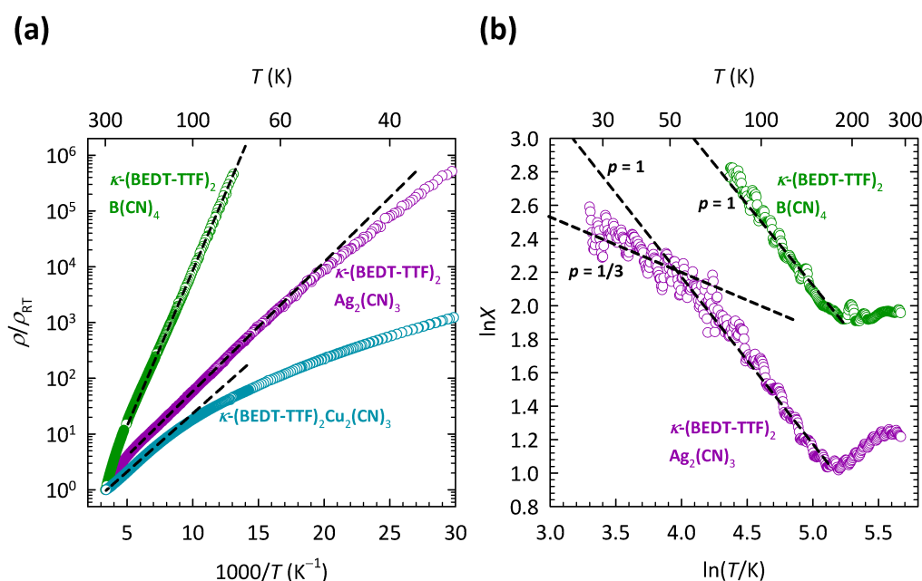
Figure 3. (a) Temperature dependence of resistivity normalized to room temperature \rho/\rho_{RT} for \kappa -(BEDT-TTF) _2 Cu _2 (CN) _3 (dark cyan symbols), \kappa -(BEDT-TTF) _2 Ag _2 (CN) _3 (violet symbols), and \kappa -(BEDT-TTF) _2 B(CN) _4 (green symbols) on a \log \rho - 1/T plot. The data for \kappa -(BEDT-TTF) _2 Cu _2 (CN) _3 are the same as in Figure 2a. Black dashed lines are fits to the NNH mechanism \rho(T) \propto \exp(\Delta_{NNH}/T) . (b) Temperature dependence of special logarithmic resistivity derivative X = -d\ln\rho/(d\ln T) = p(C/T)^p on a double logarithmic plot for \kappa -(BEDT-TTF) _2 Ag _2 (CN) _3 (violet symbols) and \kappa -(BEDT-TTF) _2 B(CN) _4 (green symbols). Black dashed lines correspond to slopes p = 1/3 for 2D VRH and p = 1 for NNH, where p is the exponent in a general expression for resistivity \rho(T) \propto \exp(C/T)^p (see text). The figure is based on data from Ref. [37].
