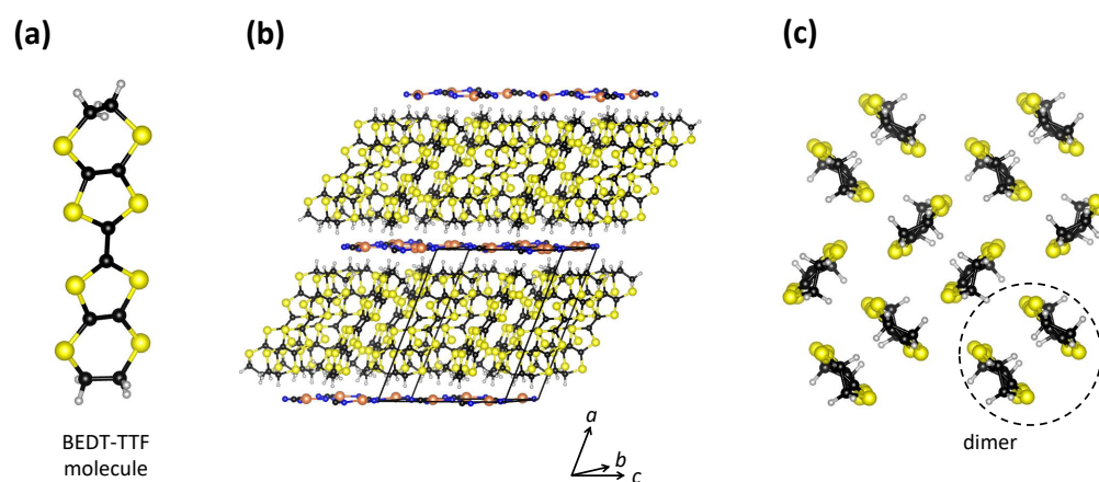
Figure 1. (a) Schematic drawing of a BEDT-TTF molecule. (b) Layered crystal structure of \kappa -(BEDT-TTF) _2 Cu _2 (CN) _3 . The unit cell is indicated by black lines. (c) View of a BEDT-TTF layer in the bc plane projected along the a axis. Sulphur, carbon, copper, nitrogen, and hydrogen atoms are shown in yellow, black, orange, blue, and gray, respectively. This figure is based on data from Ref. [29].
