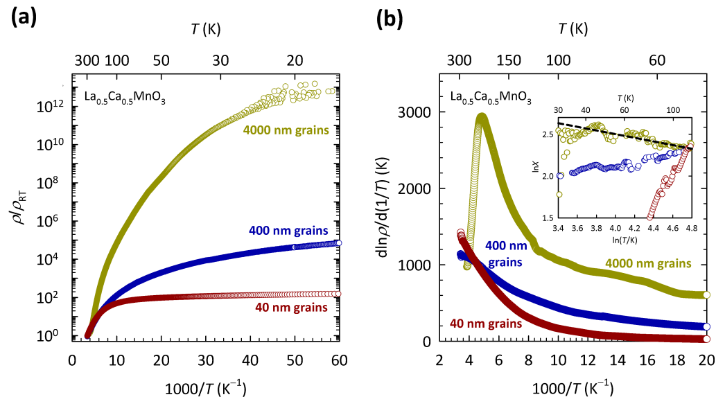
Figure 8. Temperature dependence of (a) resistivity normalized to room temperature value \rho/\rho_{\text{RT}} and (b) corresponding logarithmic resistivity derivative d \ln \rho / d \ln(1/T) for \text{La}_{0.5}\text{Ca}_{0.5}\text{MnO}_3 ceramic samples with different grain sizes: 4000 nm (dark yellow symbols), 400 nm (dark blue symbols), and 40 nm (dark red symbols). The data for the sample with 4000 nm grains are the same as in Figure 7a. Maximum in d \ln \rho / d \ln(1/T) corresponds to the CO transition (see text). Inset shows the T dependence of special logarithmic resistivity derivative X = -d \ln \rho / (d \ln T) = p(C/T)^p on a double logarithmic plot. Black dashed line corresponds to slope p = 1/4 for 3D VRH, where p is the exponent in a general expression for resistivity \rho(T) \propto \exp(C/T)^p (see text). The figure is based on data from Ref. [96].
