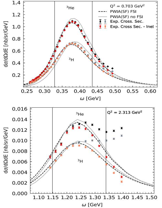
FIG. 2. Cross sections and statistical uncertainties for ^3\text{H} and ^3\text{He} compared to spectral-function calculations of Ref. [32] for the L24 ( 0.703 \text{ GeV}^2 ) and R24 ( 2.313 \text{ GeV}^2 ) settings. The black (gray) points are the measured total cross section, and the red (orange) points are after subtraction of the inelastic contribution. The vertical lines represent \pm 1\sigma from the QE peak (see text for details).
