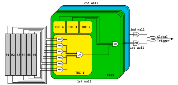
Fig. 4. Sketch of the neutron polarimeter trigger scheme. A trigger is formed for each wall (first wall indicated in green and second wall in cyan) separately and then combined to the final polarimeter trigger which is forwarded to the global A1 trigger system.
