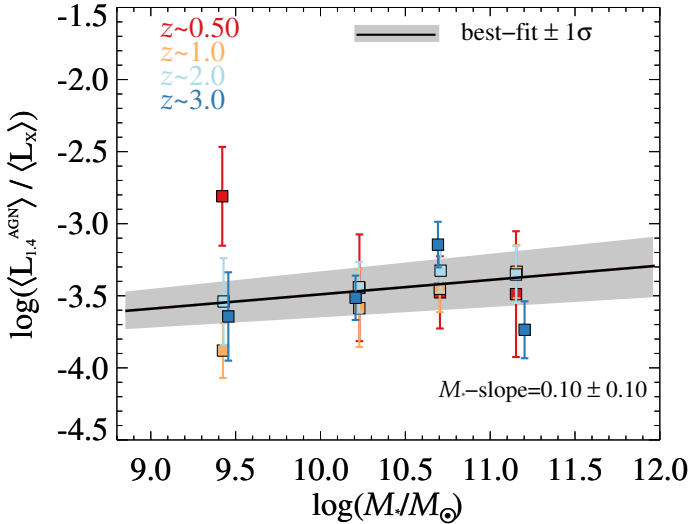
Fig. 12. Logarithmic ratio between our \langle L_{1.4}^{\text{AGN}} \rangle measurements and the \langle L_X \rangle obtained from X-ray stacking (Carraro et al. 2020), as a function of M_* , coloured by redshift. The black line indicates the best-fit ratio with M_* , by imposing a z -invariant trend, which returns a M_* -slope of 0.10 \pm 0.10 . The grey shaded area marks the \pm 1\sigma confidence interval after propagating the parameter uncertainties. See Sect. 6.4.2 for details.
