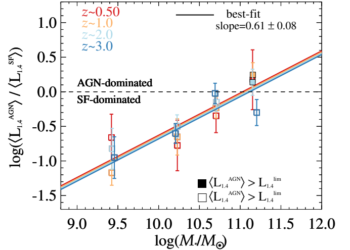
Fig. 9. Logarithmic ratio between AGN-related and SF-related radio emission ( \langle L_{1.4}^{\text{AGN}} \rangle and \langle L_{1.4}^{\text{SF}} \rangle , respectively), as a function of M_* , coloured by redshift. Each data point (square) represents the ratio between average AGN and SF luminosities for M_* -selected SFGs in the same bin. The dividing threshold between AGN and SF-dominated regions (dashed black line) is crossed at M_* \sim 10^{11} M_\odot , above which galaxy radio emission is mainly powered by AGN jets. Filled squares mark bins in which the mean \langle L_{1.4}^{\text{AGN}} \rangle is above the 5\sigma VLA 3 GHz luminosity limit ( L_{1.4}^{\text{lim}} , scaled to 1.4 GHz). Coloured lines indicate the best-fit ratio (solid) from Eq. (10).
