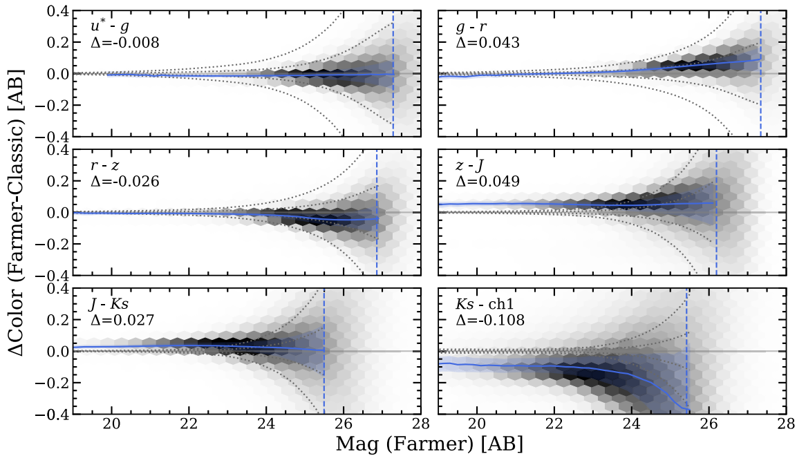
Figure 9. Comparison of broadband colors between the THE FARMER and CLASSIC catalogs, \Delta_{\text{color}} . THE FARMER magnitudes of the first color term in each panel are shown on the x-axis. Colors for individual sources are shown by the underlying density histogram, which is described by the overlaid median binned by 0.2 AB with a 68% confidence interval. 1\sigma and 3\sigma photometric uncertainty estimates on the colors are indicated by the gray dotted curves, and the mean 3\sigma depth computed from both bands of interest and measured with 3'' diameter apertures as reported in Table 1 are shown by vertical dashed lines; brighter than the median \Delta are reported.
