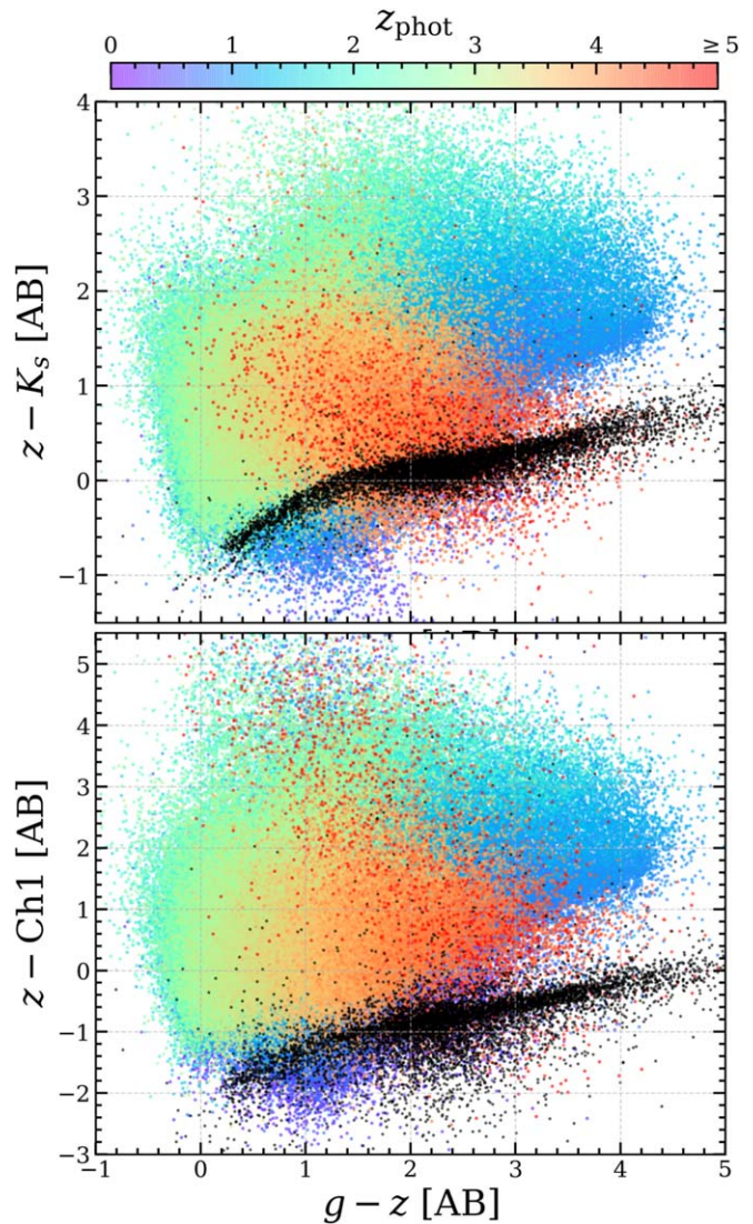
Figure 12. Color–color diagrams showing stars (black) and galaxies (colored by z_{\text{phot}} ) classified by LePhare for THE FARMER photometry, shown in g-z , K_s (top) and g-z , \text{ch1} (bottom) color–color diagrams. For simplicity, galaxies with z_{\text{phot}} > 5 are shown also by red points. Only sources with S/N > 3 in g , z , K_s , and \text{ch1} in the UltraVISTA area outside the HSC bright-star halos are shown.
