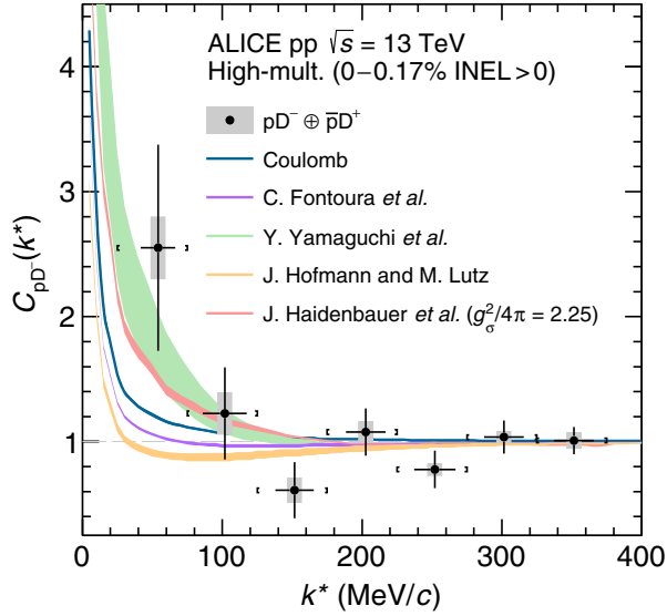
FIG. 3. Genuinely pD^- correlation function compared with different theoretical models (see text for details). The null hypothesis is represented by the curve corresponding to the Coulomb interaction only.
