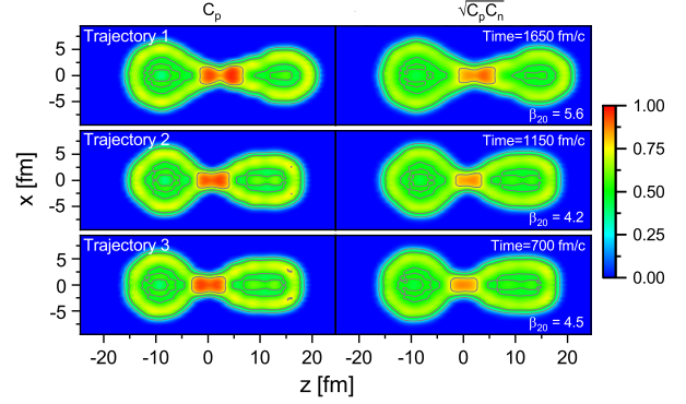
FIG. 2. The proton C_p (left) and total \sqrt{C_p C_n} (right) localization functions in the x - z coordinate plane for the three fission trajectories, at times that immediately precede scission.
