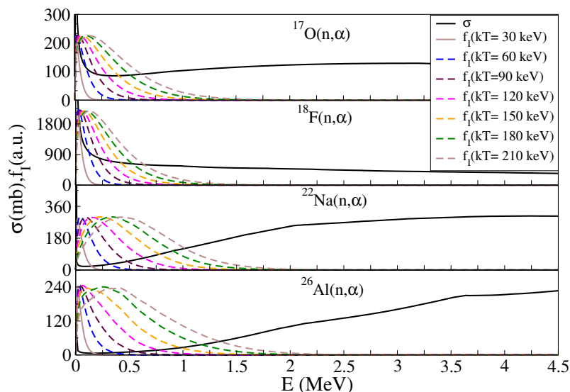
Figure 7. Relevant (n, \alpha) reaction energy windows for the range of temperatures kT = 30\text{--}210 keV described with the function f_I(E) (in arbitrary units, see text) and the respective reaction cross sections for ^{17}\text{O} , ^{18}\text{F} , ^{22}\text{Na} , and ^{26}\text{Al} target nuclei.
