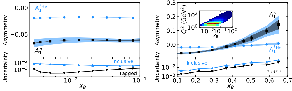
Fig. 6. A direct comparison of A_1^n extracted from inclusive measurements (blue band) and tagged measurements (black square) which are superimposed on the blue band. The left plot is for x_B \leq 0.1 and the right plot is for x_B \geq 0.1 . The blue points are the A_1^{3\text{He}} measured values from inclusive measurements from which the blue band is extracted. The uncertainties for both the techniques are compared in the bottom box where the blue (black inverted) triangles are the absolute uncertainties of inclusive (tagged) measurements. The data points were located at the average value for each x_B bin. The asymmetry calculation for each data point corresponds to the average value of Q^2 for each x_B bin.
