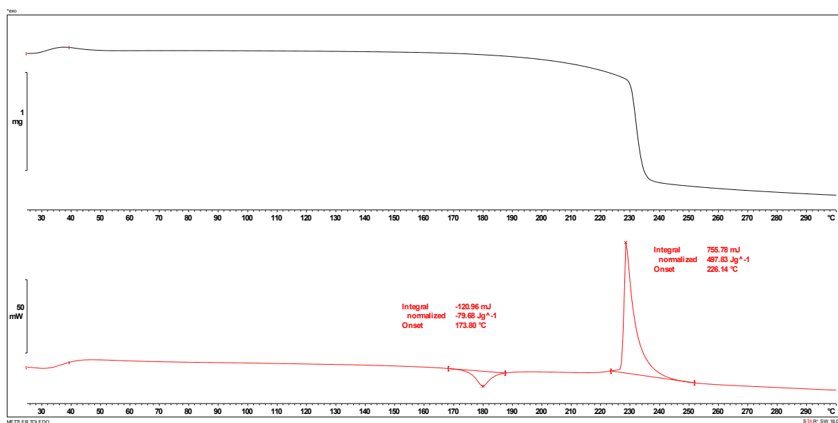
Slika D58. TG i DSC termogram soli (\text{HINZ})\text{NO}_3 .
