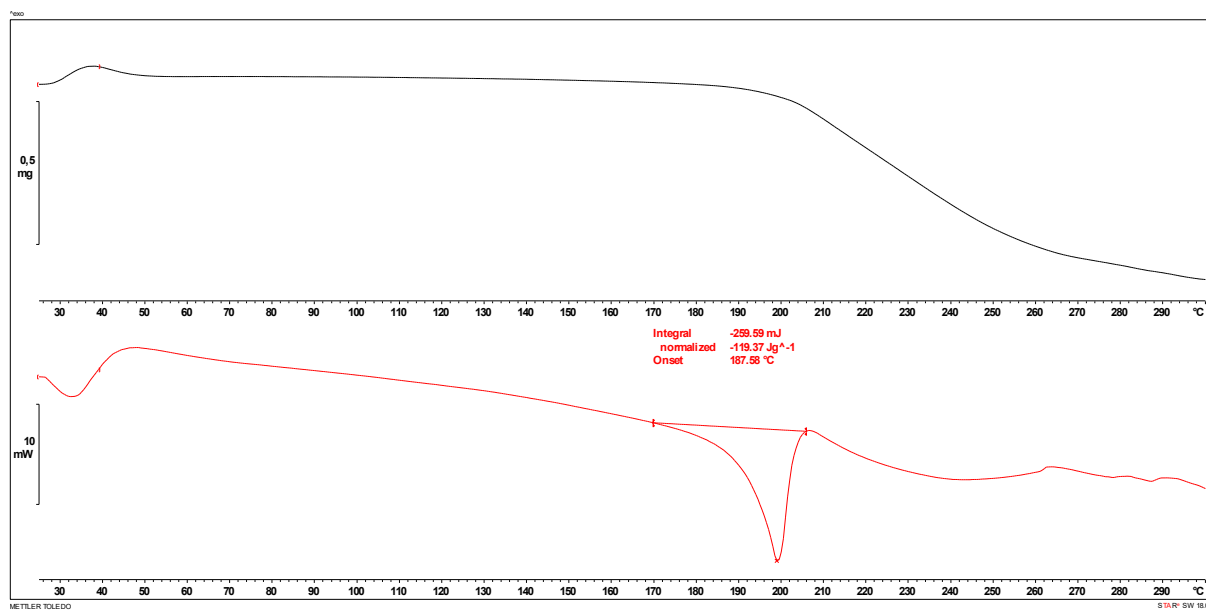
Slika D63. TG i DSC termogram soli (\text{HINZ})(\text{H}_2\text{PO}_4) .
