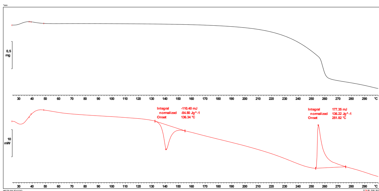
Slika D57. TG i DSC termogram soli (\text{HNZ})\text{NO}_3 .
