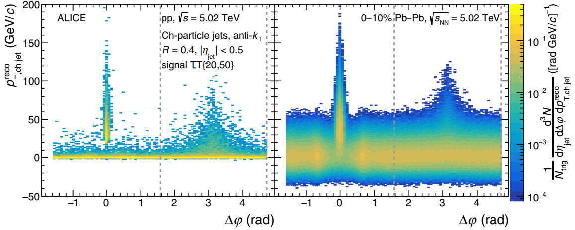
FIG. 1. Trigger-normalized recoil jet distributions ( R = 0.4 ) as a function of \Delta\varphi and p_{T,\text{ch jet}}^{\text{reco}} , in pp collisions (left) and in Pb-Pb collisions (right) at \sqrt{s_{\text{NN}}} = 5.02 TeV, for \text{TT}\{20, 50\} GeV/c. The azimuthal region of the analysis is indicated by the vertical dashed lines.
