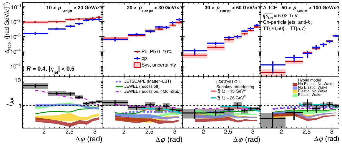
FIG. 20. Same as Fig. 19, for R = 0.4 .
