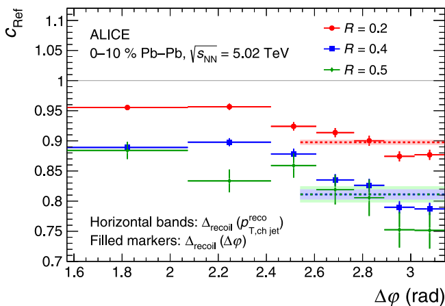
FIG. 5. Scaling factor c_{\text{Ref}} of \Delta_{\text{recoil}}(\Delta\phi) for R = 0.2, 0.4 , and 0.5 . The vertical bars indicate the statistical uncertainties. The value of c_{\text{Ref}} for the \Delta_{\text{recoil}}(p_{T,\text{jet}}^{\text{reco}}) analysis, which integrates over the region |\Delta\phi - \pi| < 0.6 , is displayed as a horizontal bar for each value of R , with shaded bands indicating statistical uncertainty.
