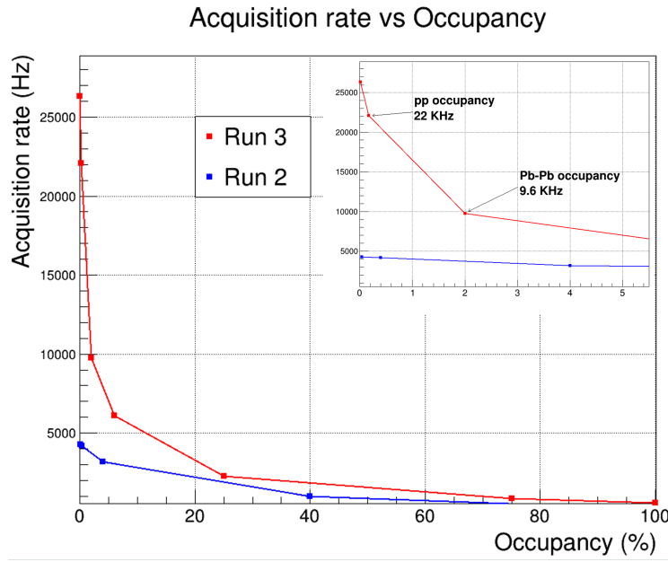
Figure 79. Event rate as a function of the detector occupancy, which is on average about 0.17% and 2% in pp and Pb-Pb collisions, respectively.
