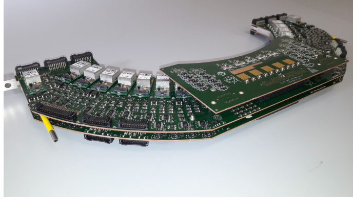
Figure 42. MFT PSU boards with mezzanine assembled on their support.
