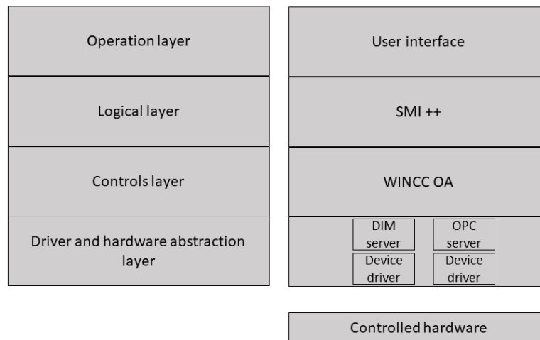
Figure 100. DCS software architecture.
