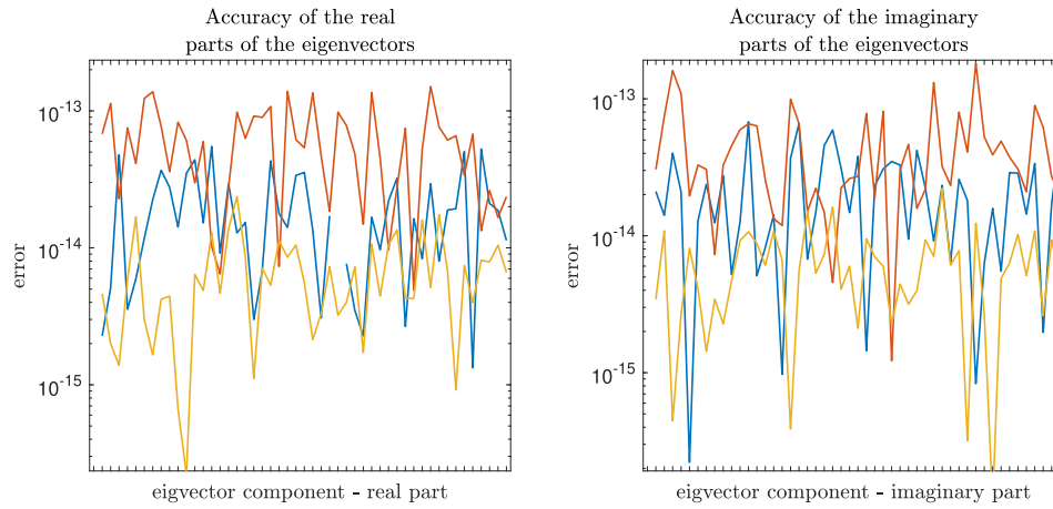
Figure 2.5: Accuracy of the eigenvectors from the Eberlein method in comparison to the Matlab eig function.
