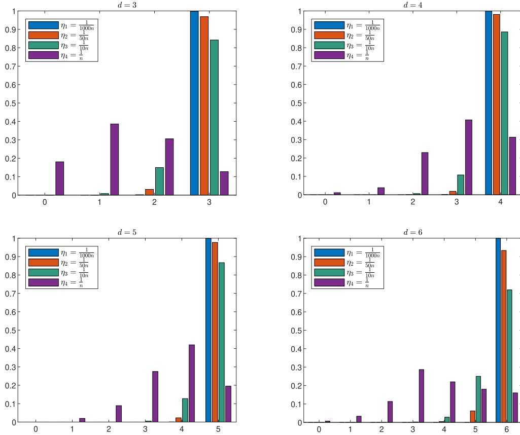
Figure 4.6: Portion of the number of microiterations within one iteration for different values of \eta on random tensors of order d = 3, 4, 5, 6 .
