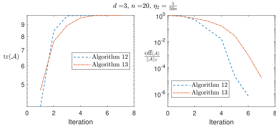
Figure 4.11: Convergence of Algorithms 12 and 13 on a tensor of order 3 that is diagonalizable using orthogonal transformations.
