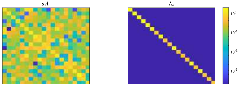
(b) The starting matrix d\mathbf{A}_4 and fully diagonal matrix \Lambda_d obtained from the block Eberlein algorithm.
