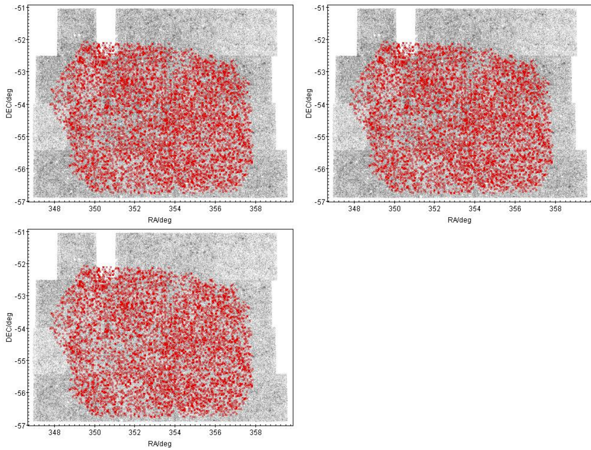
Figure 2.3: Overlap between positions of the NIR sources, noted in black and positions of radio sources, noted in red. From top left to bottom, the bands are: J , H and K
