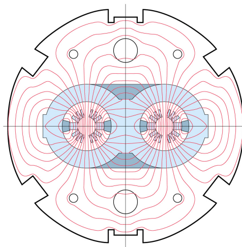
Computed magnetic flux map at B_0=10 Tesla
