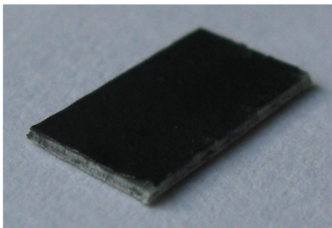
Figure 8.1: Film of the PD2.06MC40 blend on FR4 substrate board. The board is 350 \mu\text{m} thick, and the film thickness is 9 \mu\text{m} .
