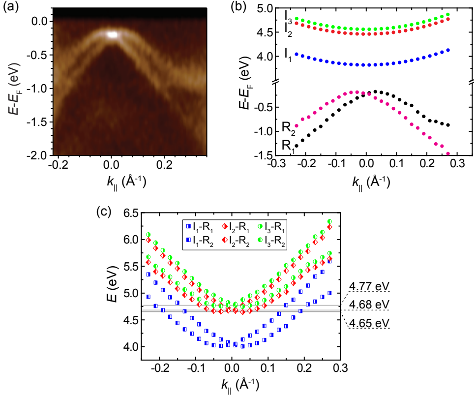
Figure 4.3: (a) ARPES spectra of the Rashba-split surface state of Gr/Ir(111). EDC-ARPES, \parallel GK, \hbar\omega = 55 eV, p -polarization, T_S = 75 K. (b) Data points from EDC analysis of the spectrum in (a) ( R_1 and R_2 ) and data points representing first three IP states ( I_1 , I_2 and I_3 ) plotted according to Ref. [134]. (c) Energy difference of the image-potential and surface states I_n - R_m ( n = 1, 2, 3 , m = 1, 2 ). Several pump-photon energies used in our experiments are marked by gray horizontal lines. Resonant transition is achieved when the difference I_n - R_m coincides with the pump-photon energy.
