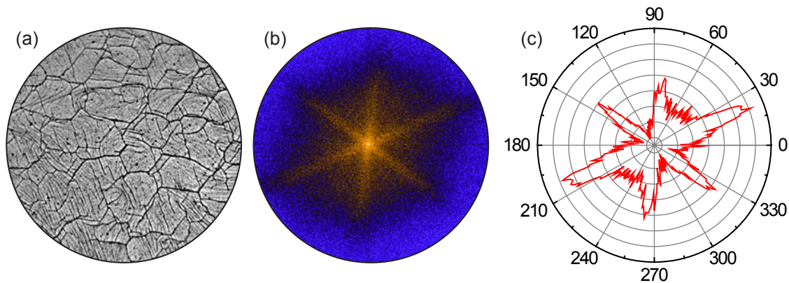
Figure 3.10: (a) LEEM image of a full graphene layer on Ir(111). Thick dark lines extending over the entire sample surface are graphene wrinkles. FOV = 9.3 \mu\text{m} , E = 16 \text{ eV} , T_S = 369 \text{ K} . (b) Fourier transform of (a). 6-fold symmetric pattern is visible corresponding to three dominant directions of wrinkle extension (c) Polar plot of radial sums extracted from (b) exhibiting 6-fold symmetry. The radial distance of the red curve is in arbitrary units.
