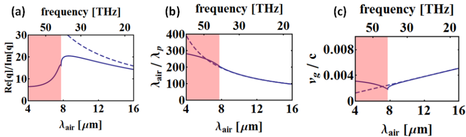
Figure 3.3: Properties of plasmons in doped graphene. Solid-lines are obtained with the number-conserving RPA calculation, and the dashed lines with the semiclassical approach. Losses (a), field localization (wave "shrinkage") (b), and group velocity (c) for doping E_F = 0.135 eV, and relaxation time \tau = 1.35 \times 10^{-13} s, which corresponds to the mobility of 10000 \text{ cm}^2/\text{Vs} . The upper scale in all figures is frequency \nu = \omega/2\pi , whereas the rose shaded areas denote the region of high interband losses.
