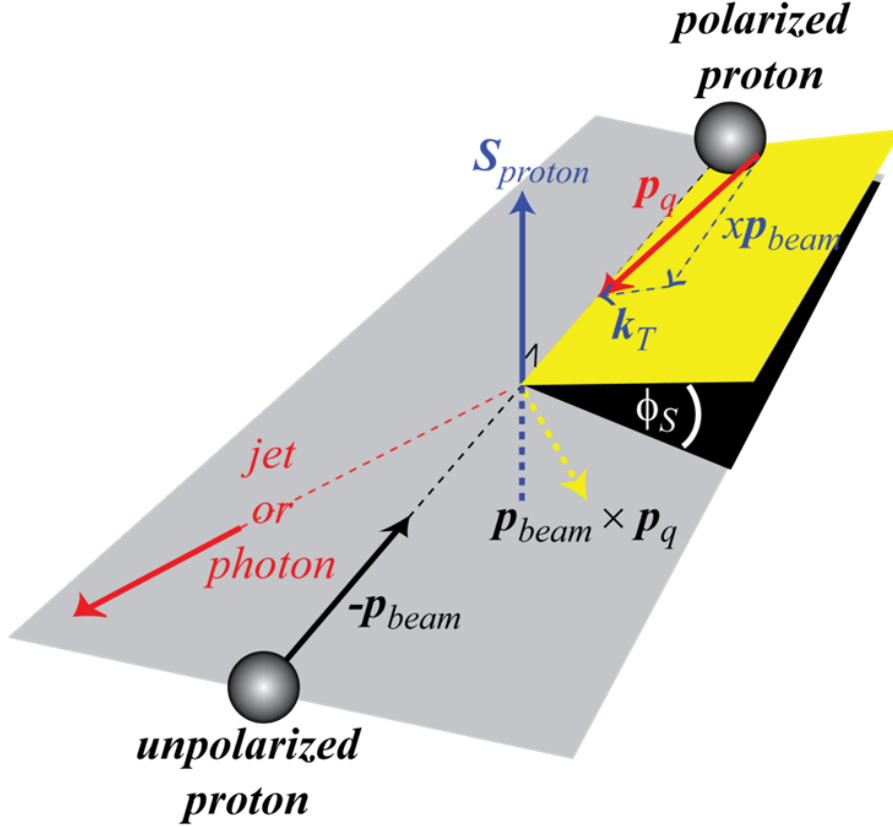
Figure 2.7: The schematic view of the Sivers variables. The Sivers angle, given earlier in the text, is the angle the quark impulse closes with the hadron collision plane perpendicular to the spin of the proton.
