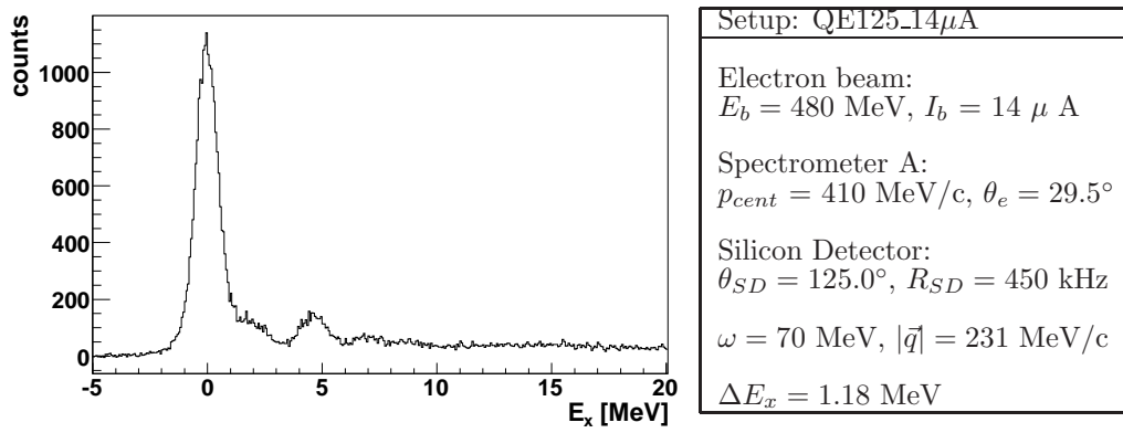
Figure 5.7: Excitation spectrum of ^{11}\text{B} in kinematic setup QE125_14 \mu\text{A} .
