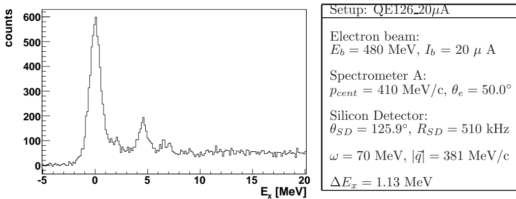
Figure 5.8: Excitation spectrum of ^{11}\text{B} in kinematic setup QE126_20 \mu\text{A} .
