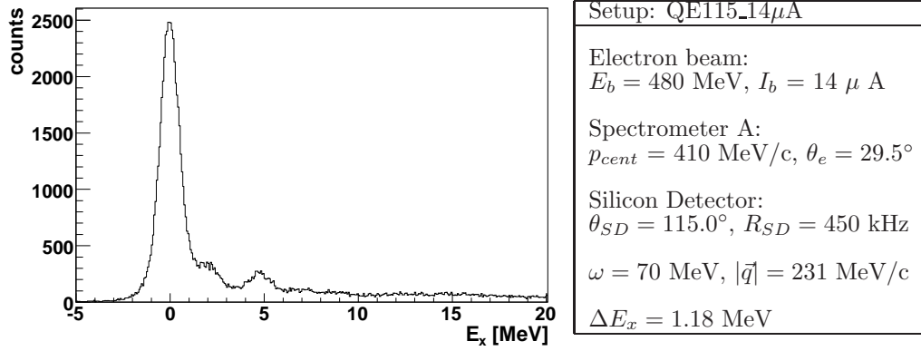
Figure 5.6: Excitation spectrum of ^{11}\text{B} in kinematic setup QE115_14 \mu\text{A} .
