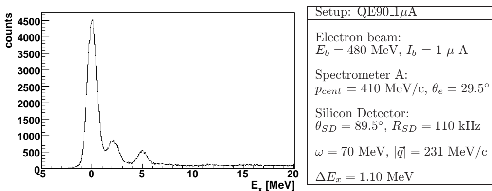
Figure 5.3: Excitation spectrum of ^{11}\text{B} in kinematic setup QE90_1 \mu\text{A} .
