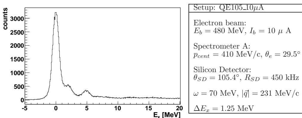
Figure 5.5: Excitation spectrum of ^{11}\text{B} in kinematic setup QE105_10 \mu\text{A} .
