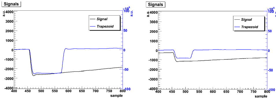
Figure B.2: Digitized preamplifier signal with the reconstructed trapezoids. The left picture shows the longer trapezoidal shaping applied for larger signals, while the shorter shaping is applied for smaller signals on in the right picture.
