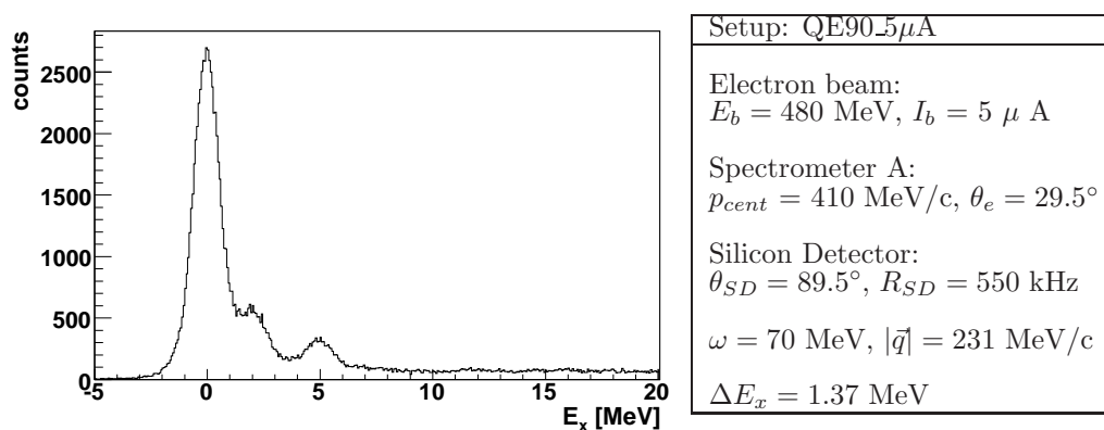
Figure 5.4: Excitation spectrum of ^{11}\text{B} in kinematic setup QE90_5 \mu\text{A} .
