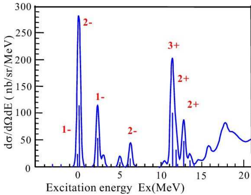
FIGURE 5.7: CALCULATED SPECTRUM FOR THE {}^{12}\text{C}(e, e'K^+){}_{\Lambda}^{12}\text{B} REACTION AT E_{\gamma} = 1.3 GEV AND \theta_{K^+}^{LAB} = 3^{\circ} WITH FIXED ENERGY RESOLUTION OF 300KEV (FWHM). UPDATE WITH NSC97F FROM [94] [95].
