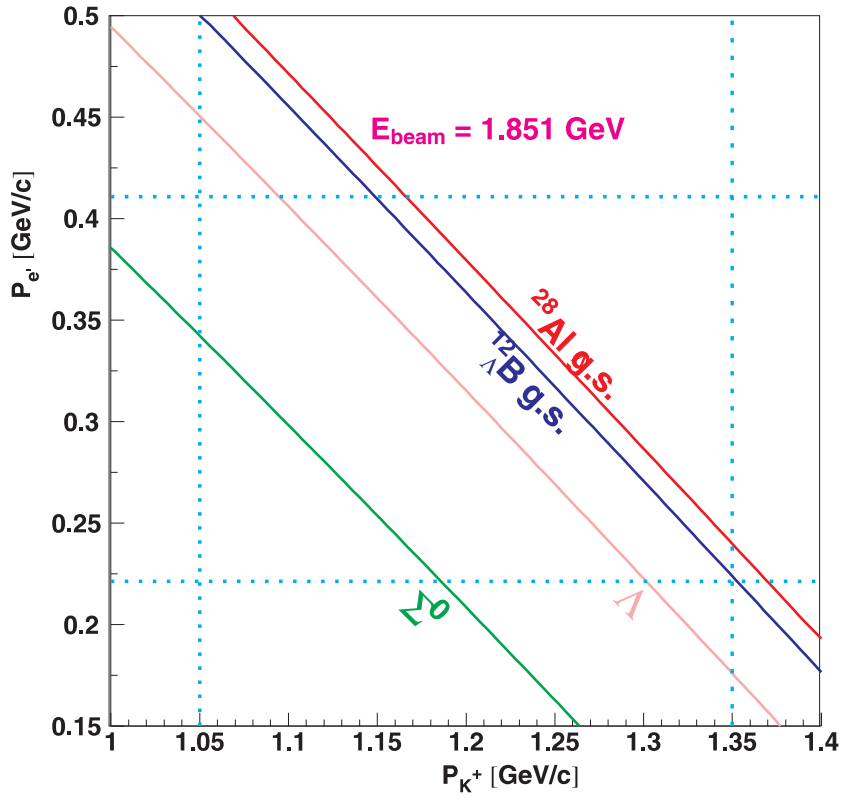
FIGURE 2.3: MOMENTUM ACCEPTANCE OF KAON AND SCATTERED ELECTRON SPECTROMETERS. ( IT IS CALCULATED WITH: BEAM ENERGY 1.851 GeV, ASSUMED BINDING ENERGY OF \Lambda B GROUND STATES -11.37 MEV [82] AND \Lambda Al GROUND STATE -16.92 MEV [58].)
