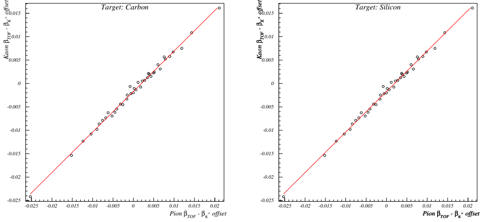
FIGURE 4.4: DEPENDENCE OF THE KAON BETA OFFSET ON PION BETA OFFSET. THIS CORRECTION WAS USED TO GET BETTER KAON/PION SEPARATION.
