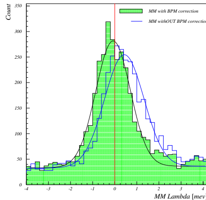
FIGURE 4.34: LAMBDA MM SPECTRA FOR TWO \text{CH}_2 DATA SETS WITH DIFFERENT BPM-IPM307X CONDITIONS. MASS OF \Lambda SUBTRACTED FROM MM SPECTRA.
