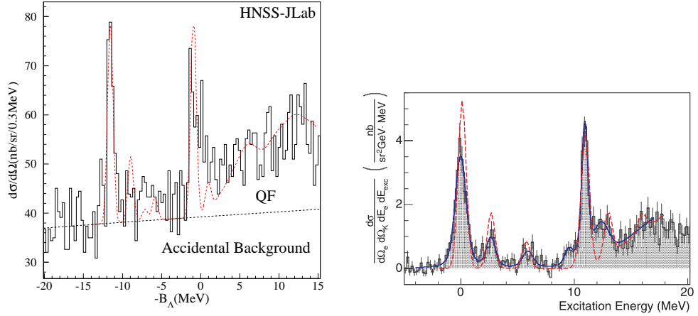
(a) JLab Hall C : E89-009 [17]
