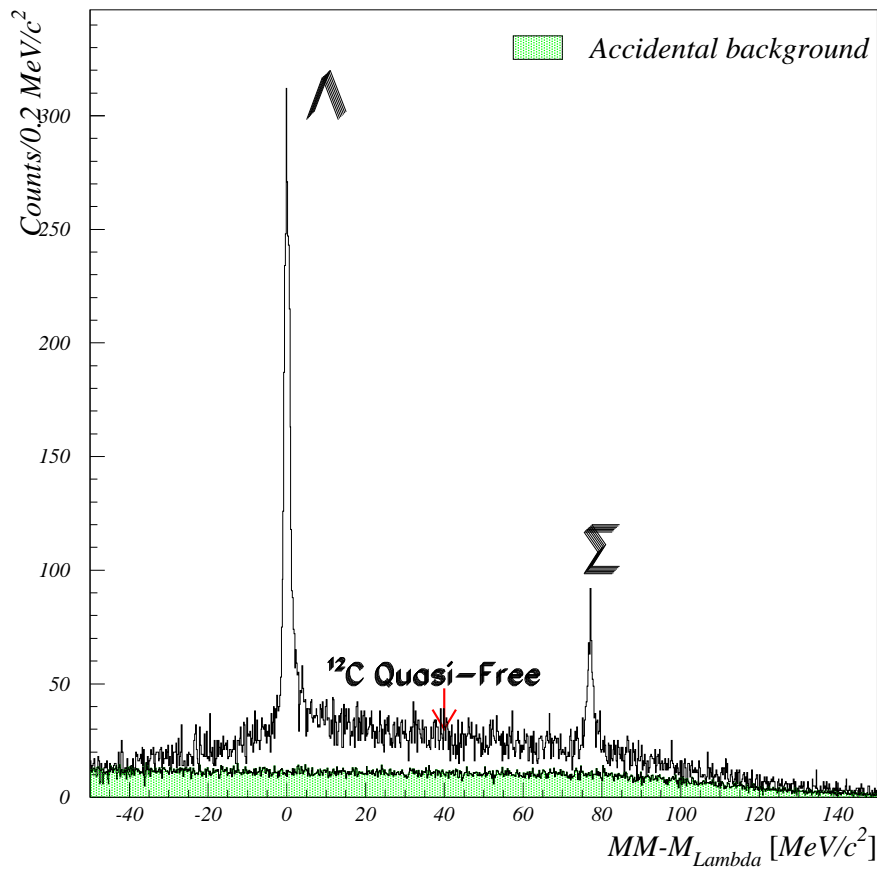
FIGURE 4.23: MISSING MASS SPECTRA FROM CH 2 DATA. \Lambda AND \Sigma PEAKS ARE CLEARLY SEEN. ACCIDENTAL COINCIDENCES AND QUASI-FREE CONTRIBUTION FROM 12 C ARE ALSO SHOWN.
