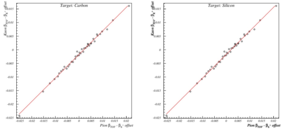
(a) Meta ^{12}\text{C}
