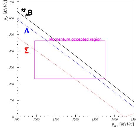
FIGURE 4.40: ENGE AND HKS MOMENTUM CORRELATION. CALCULATED FROM EQN. 4.8 FOR \Lambda , \Sigma AND ^{12}_{\Lambda}\text{B} GROUND STATE WITH BEAM ENERGY E_e = 1.853 AND SCATTERING ANGLE VALUES: \theta_{eK^+} = 0.119\text{rad} AND \theta_{ee} = 0.065\text{rad}
