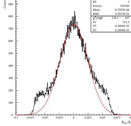
FIGURE 3.11: HKS KAON \Delta\beta = \beta_{TOF} - \beta_K DISTRIBUTION FOR THE CH_2 DATA.
