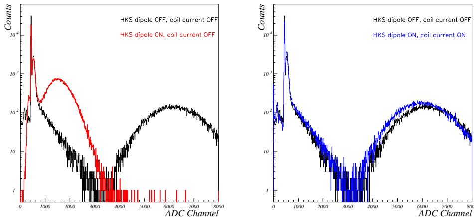
FIGURE 2.37: Left , EFFECT OF THE FRINGE FIELD ON THE PERFORMANCE OF THE AC PMTs. Right RECOVERED PERFORMANCE OF THE AC PMT WITH COILED WIRE INDUCED FIELD THAT CANCELED HKS DIPOLE FRINGE FIELD.
