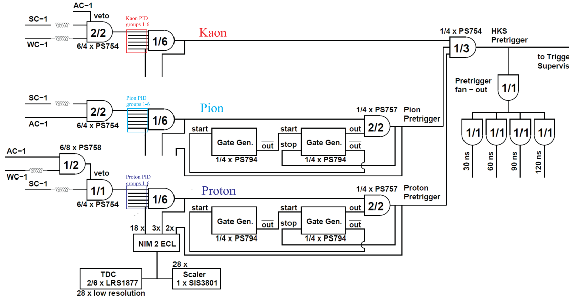
FIGURE 2.43: THE HKS TRIGGER LOGIC.
