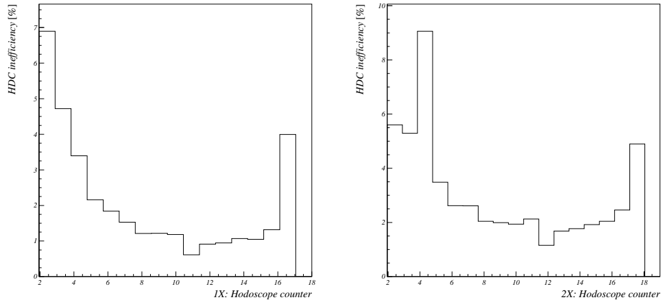
FIGURE 3.27: HDC TRACKING INEFFICIENCY ACROSS HTOF1X AND HTOF2X HODOSCOPE PLANES FOR THE \text{CH}_2 TARGET.
