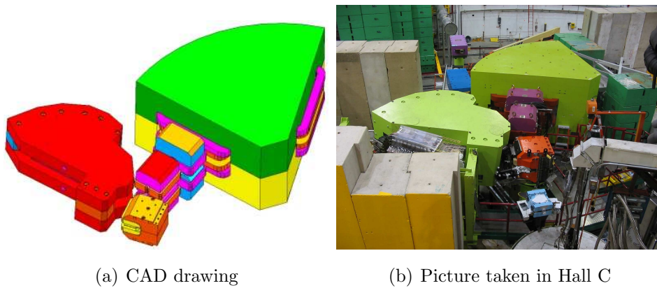
FIGURE 2.12: 3D OVERVIEW OF THE E01-011 SPECTROMETER SYSTEM: SPLITTER MAGNET, ENGE AND HKS SPECTROMETERS.
