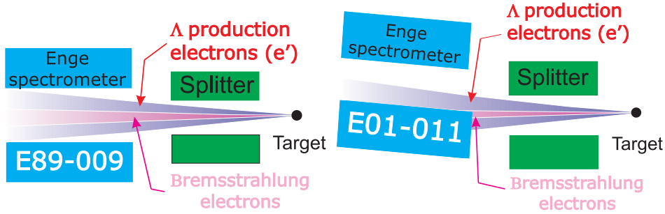
(a) Enge configuration used in E89-009. (b) Enge configuration used in E01-001.
