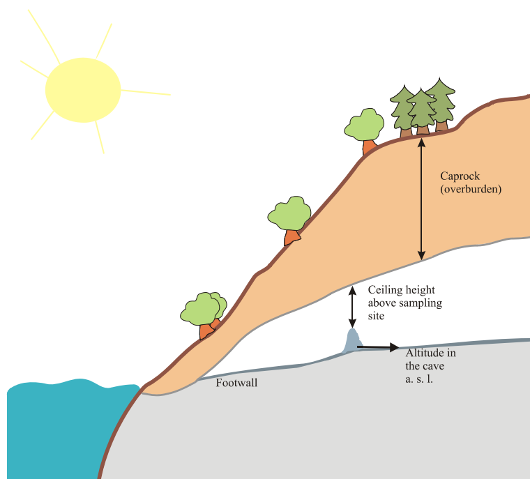
Figure 5.3 Schematic view of terms used in site description in Table 5.1.
