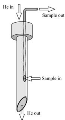
Figure 2.10 Double-hole sampling needle
