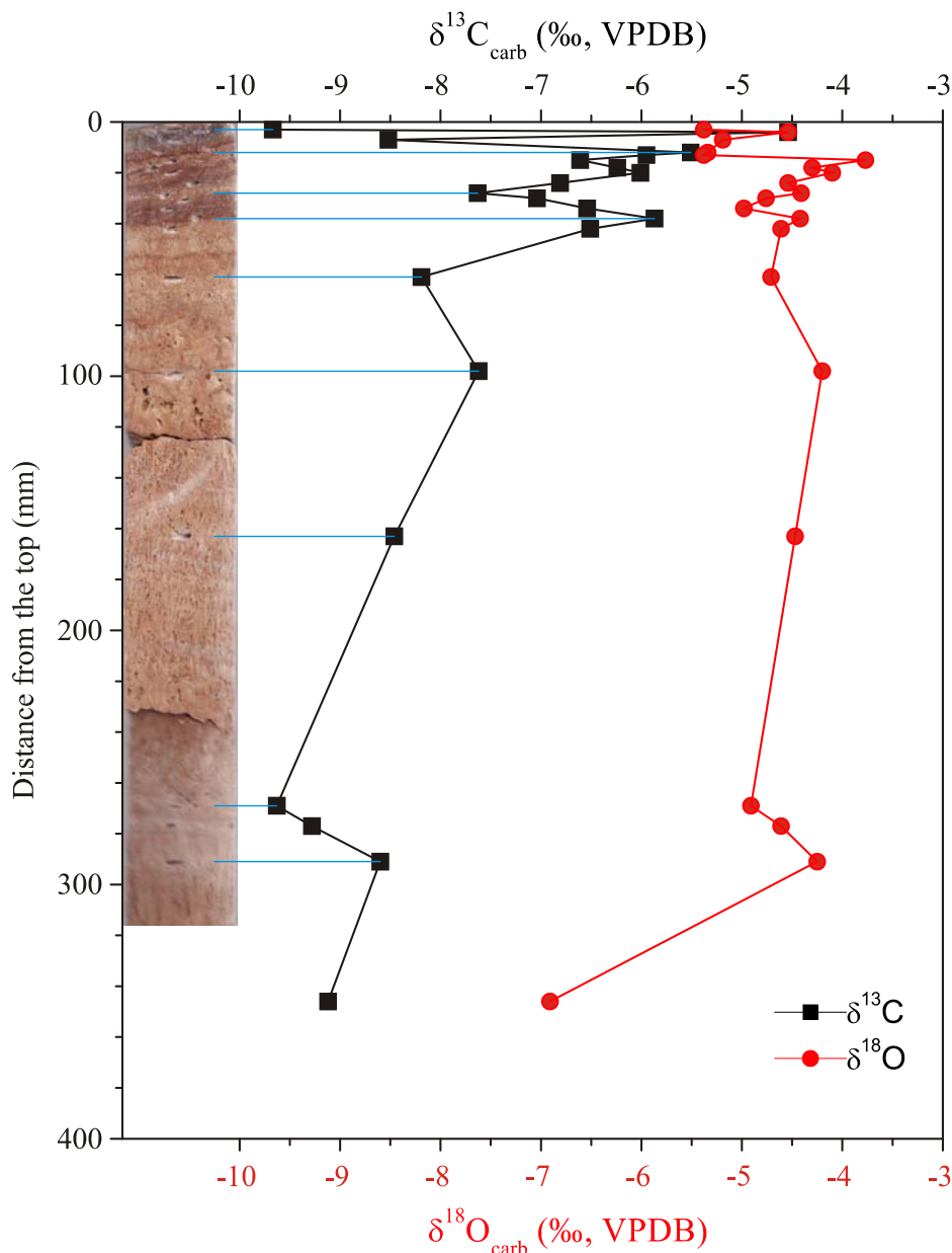
Figure 7.40 Stable isotope composition, \delta^{13}\text{C} and \delta^{18}\text{O} , along the vertical profile of the drilled core of the stalagmite from location 07 – Čarobni vrt. Blue lines are plotted only to guide an eye i.e. connect place of drilling with measured stable isotope value.
