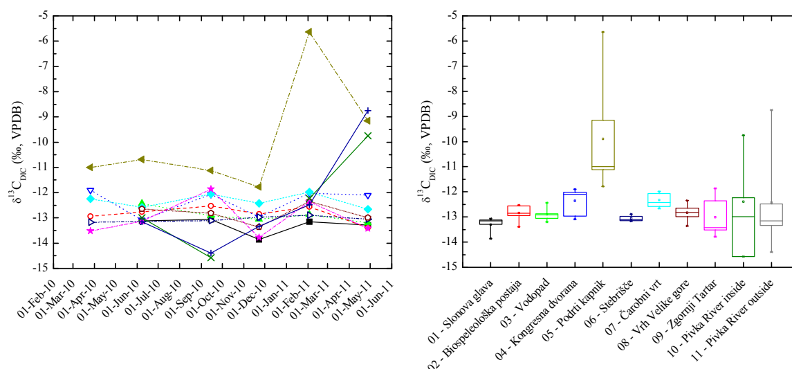
Figure 7.15 \delta^{13}\text{C}_{\text{DIC}} in drip water and River Pivka.
