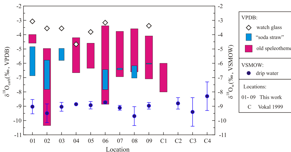
Figure 7.34 \delta^{18}\text{O} of drip water and carbonates at different sampling locations. Slika 7.34 \delta^{18}\text{O} prokapičnice i karbonata na raznim lokacijama uzorkovanja.
