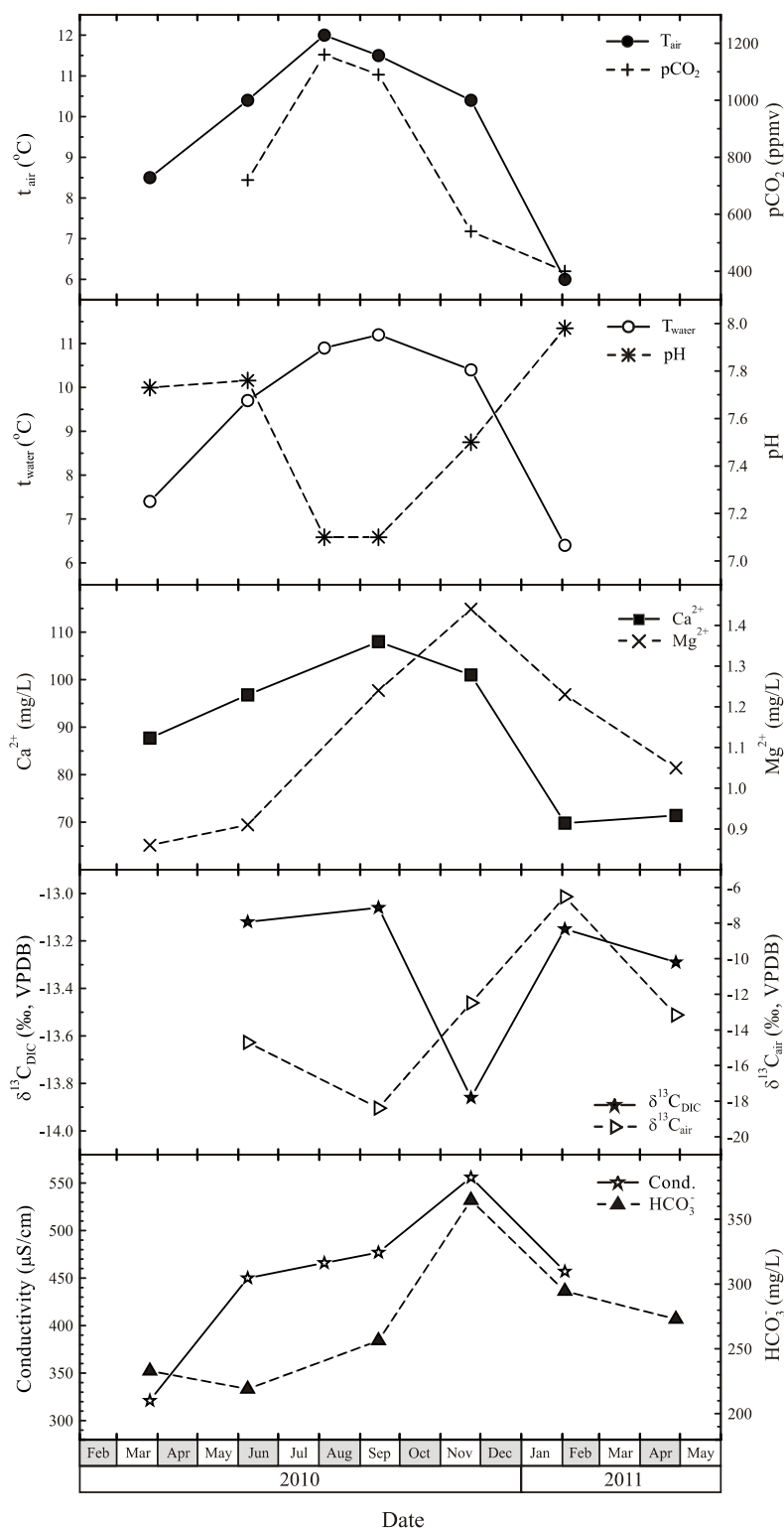
Figure 6.1 Time series of field measured parameters (air temperature, water temperature, pH, conductivity, and p\text{CO}_2 ), chemical parameters ( \text{Ca}^{2+} , \text{Mg}^{2+} , and \text{HCO}_3^- concentrations) in drip water and stable isotope composition \delta^{13}\text{C}_{\text{DIC}} and \delta^{13}\text{C}_{\text{air}} for location 01 – Slonova glava.
