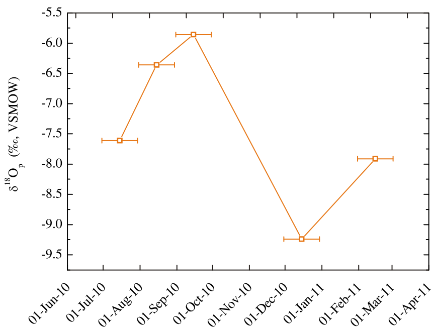
Figure 6.14 \delta^{18}\text{O} in precipitation at Postojna in the period July 2010 – March 2011.
