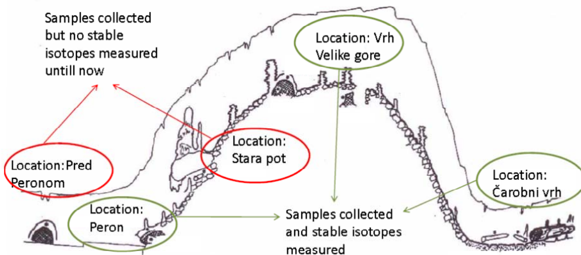
Figure 5.16 Locations where drilling of speleothems has been done (cross section). Samples from two locations, Pred Peronom and Stara pot, has not yet been analyzed.
