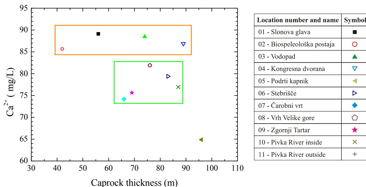
Figure 7.13 Mean values of calcium ion concentration and caprock thickness. There are two groups of locations. Red square points out outer locations and green square inner locations. Location 05 does not belong to any of the two groups
