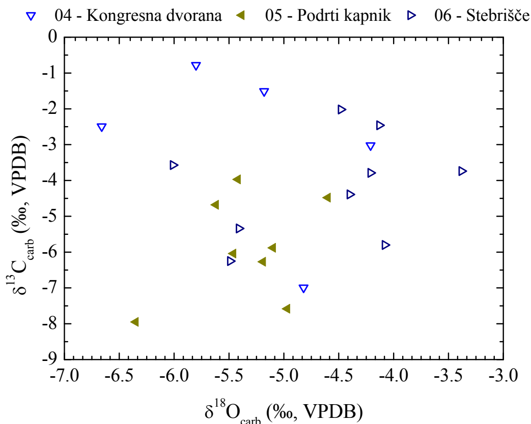
Figure 6.18 The \delta^{13}\text{C} and \delta^{18}\text{O} values of flowstones from locations 04 – Kongresna dvorana, 05 – Podrti kapnik and 06 – Stebrišče.
