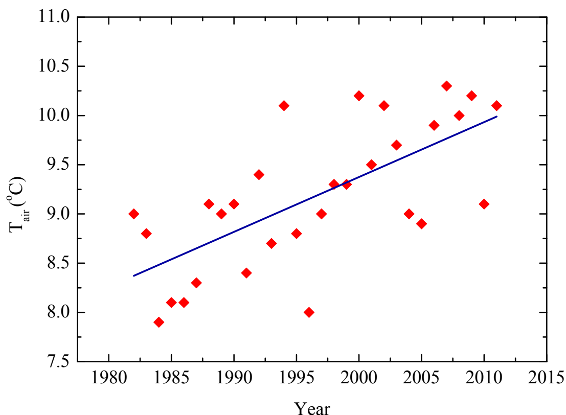
Figure 4.7 Mean yearly temperature in Postojna (♦) in the period 1982 – 2011. The slope of the linear regression line (—) is (0.056 \pm 0.011) ^\circ\text{C}/\text{yr} , R = 0.67 . Data from National Meteorological Service of Slovenia (meteo.si).
