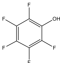
pentafluorfenol
