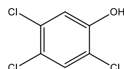
2,4,5-triklorfenol
