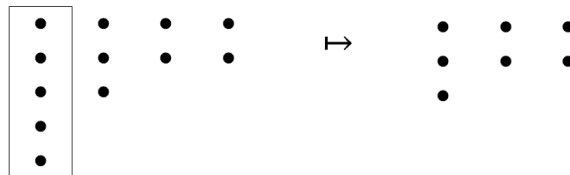
Slika 5: (4, 4, 2, 2, 1) \mapsto (3, 3, 1)
