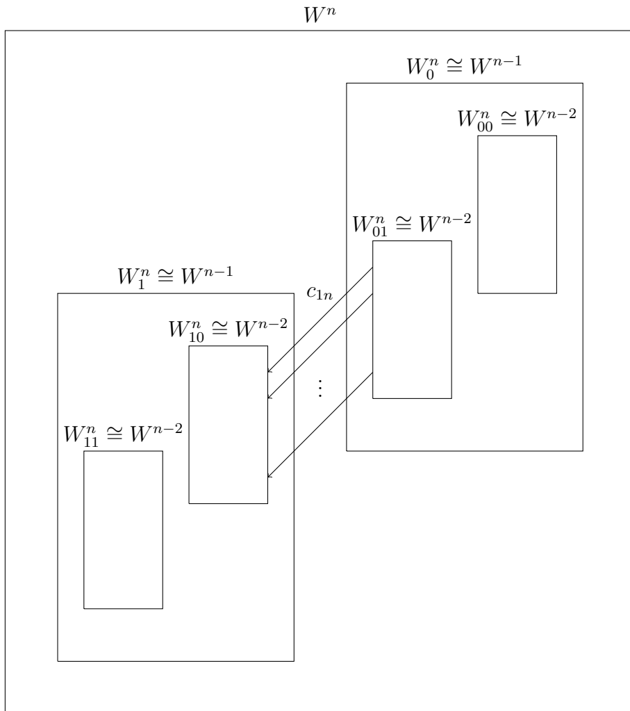
Figure 4.6: Inductive structure of W^{\mathbf{p}} for \mathbf{p} = \circ - \circ \cdots \circ - \circ \leftarrow \times
