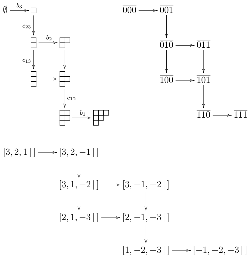
Figure 4.3: W^p and W^p\rho for p = o - o \leftarrow x
