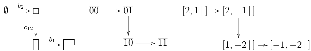
Figure 4.2: W^p and W^p\rho for p = o \leftarrow x
