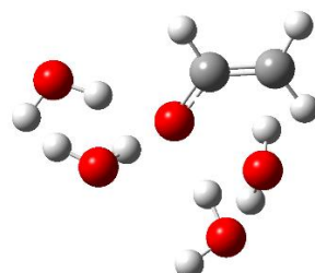
\text{CH}_2=\text{CH}-\text{O}^- -4-6 (2,16)
