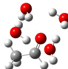
CH 3 CH=O-4-6 (0,80)
