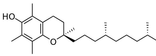
\alpha -TOH
