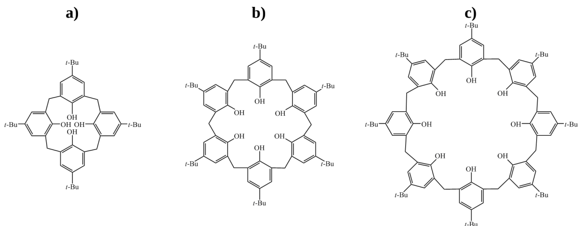
Slika 4. Predstavnic kaliksarena: a) p - tert -butilkaliks[4]aren, b) p - tert -butilkaliks[6]aren, c) p - tert -butilkaliks[8]aren.
