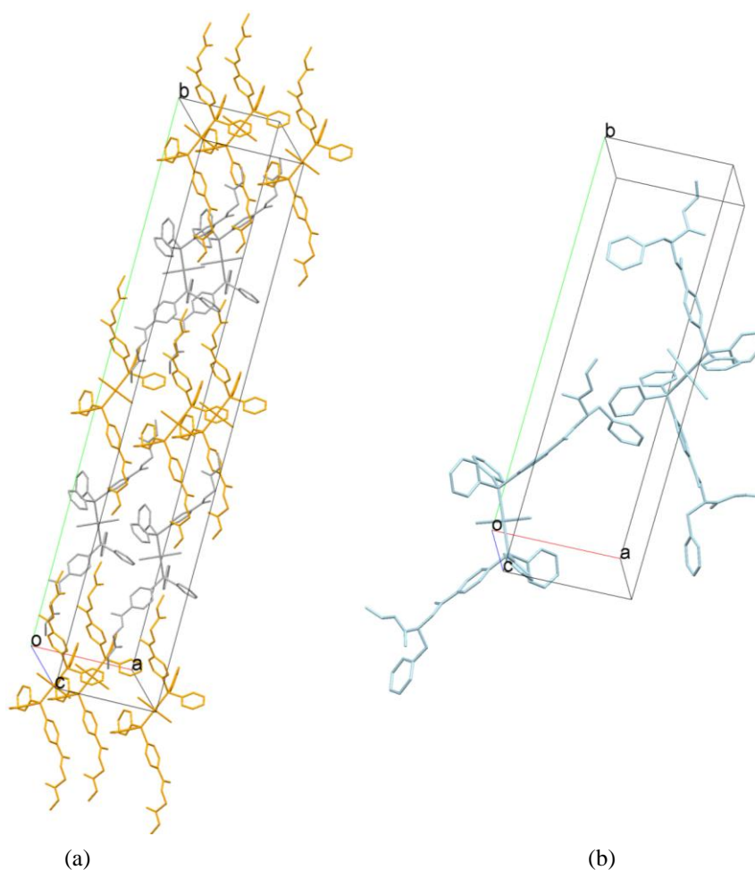
Slika 72. Kristalno pakiranje kompleksa \text{trans}-[\text{PdCl}_2(\mathbf{L})_2] s ligandima (a) \mathbf{A1a} i (b) \mathbf{A1m} .
