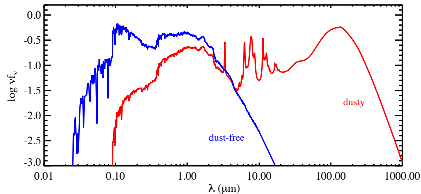
Figure 1.3: Galaxy spectral energy distribution example from near UV to mm wavelengths (reproduced from Conroy, 2013). The blue line represents a dust-free galaxy, while the the red one includes emission and attenuation by dust.
