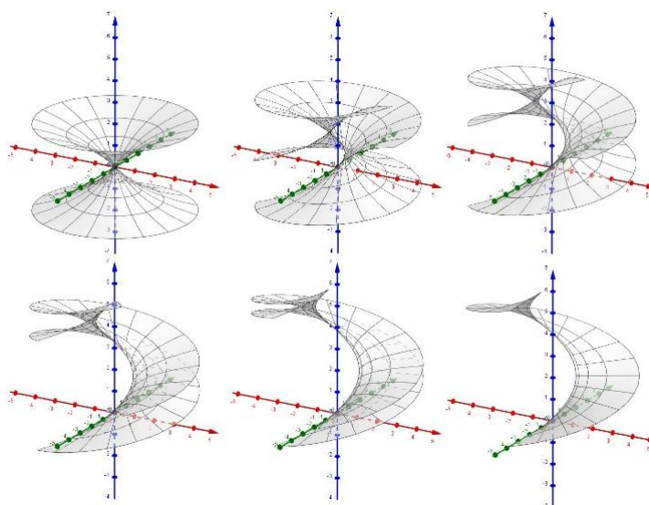
Slika 2.7: Plohe iz asociране familije katenoida y^2 + z^2 = \operatorname{sh}^2 x za \theta \in \left\{0, \frac{\pi}{10}, \frac{\pi}{5}, \frac{3\pi}{10}, \frac{2\pi}{5}, \frac{\pi}{2}\right\}
